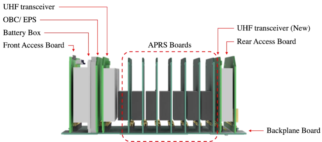
Figure 3 Internal configuration of the satellite
