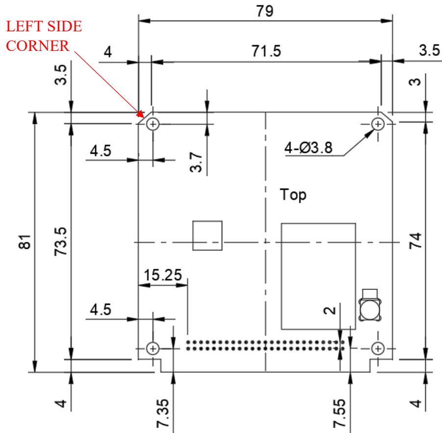
Figure 8 APRS payload board size requirements: top view
