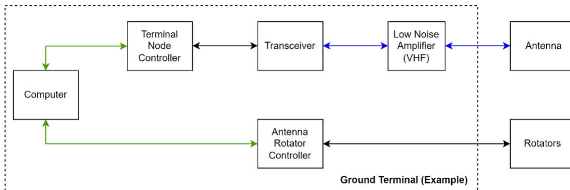
Figure 1. Ground Terminal Schematic (Not mandatory)
